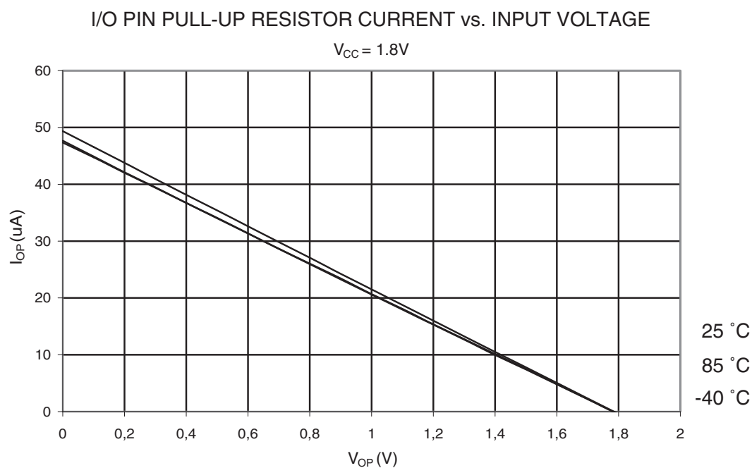
Figure 20-13. I/O Pin pull-up Resistor Current vs. Input Voltage ( V_{CC} = 1.8V )
